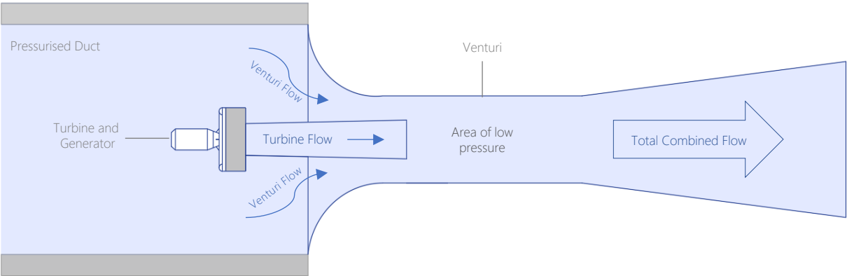
The turbine discharges into a very low pressure region created by the venturi flow. The pressure differential across the turbine therefore increases as the turbine not only experiences the site head pressure but also the considerably lower venturi pressure downstream of the turbine.
